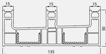
Triple Rail Profile(I-75) 41221 - 02000
