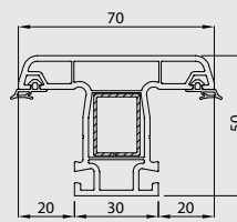
Mullion Profile 41150-13000
