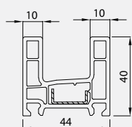
Double Rail Profile(I-44) 41231-02000
