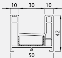
Double Rail Profile(I-50) 40502-11000
