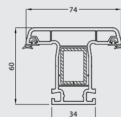
Mullion Profile 41101 - 12000
