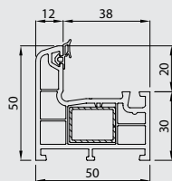
Frame Profile 41150-11000
