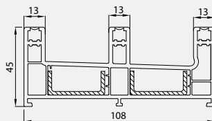
Triple Rail Profile(I-60) 41201 - 15000
