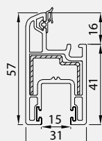
Sash Profile(I-50) 40502-13000
