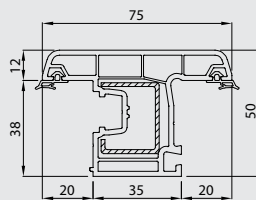
Sash Profile 41150-12000
