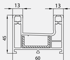
Double Rail Profile(I-60) 41201 - 12000
