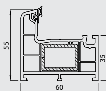
Frame Profile 41101 - 11000
