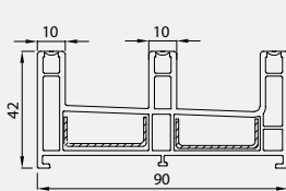
Triple Rail Profile(I-50) 40502-15000
