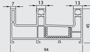
Double Rail with Screen Track Profile(I-60) 41201-15100
