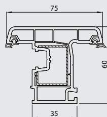
Window Sash Profile 41101 - 13000
