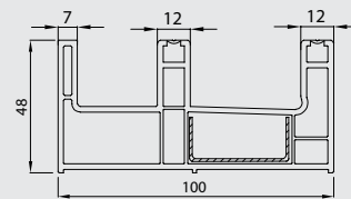
Double Rail with Screen Track Profile(I-64) 41164-10200
