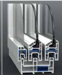
Double Rail with Screen Sash
