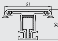
Sash/Mullion profile 41201-04000
