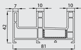
Double Rail with Screen Track Profile(I-50) 40502-12000
