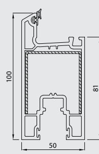
Mega Sash Profile(I-75) 41221-14000
